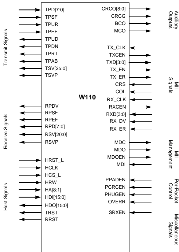
Figure 1. Logic Symbol
