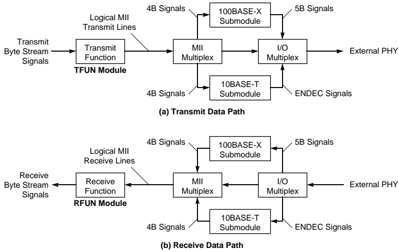
Figure 7. Transmit and Receive Data Paths
